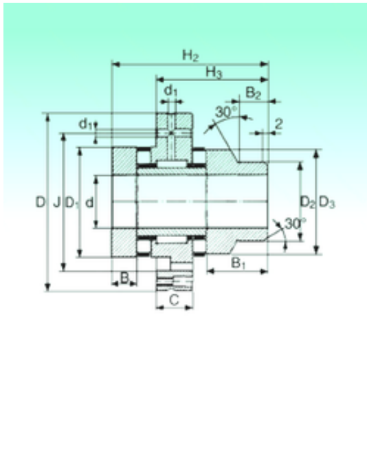
ZARF 3080 L TN Bearing 2D drawings and 3D CAD models
