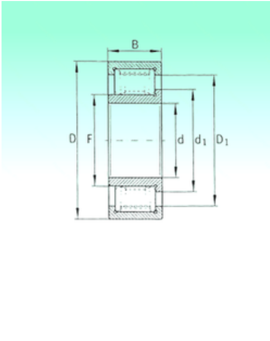
ZSL192318 Bearing 2D drawings and 3D CAD models
