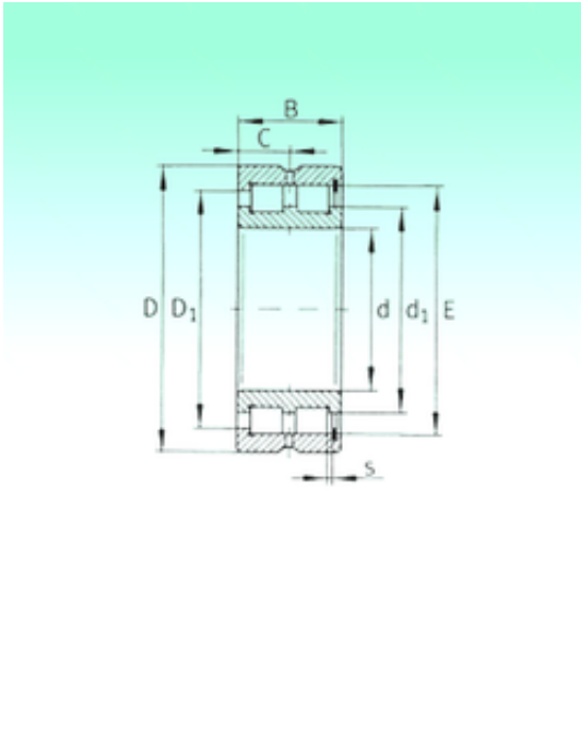
SL185007 Bearing 2D drawings and 3D CAD models
