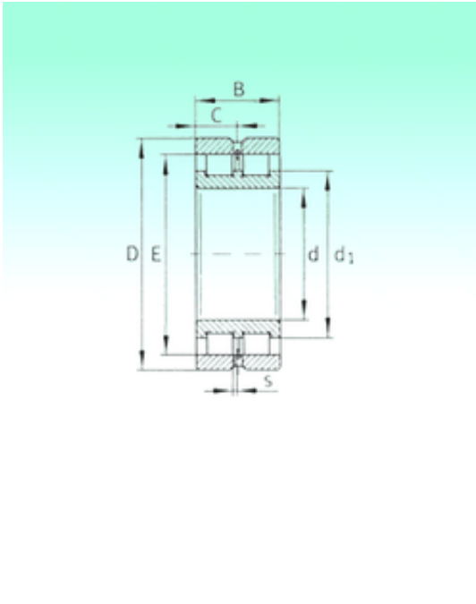
SL024960 Bearing 2D drawings and 3D CAD models
