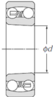
Tapered bore
