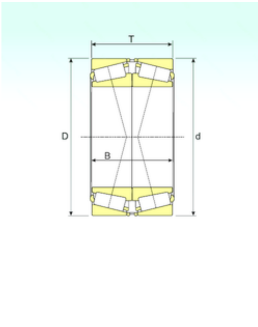
31328XJ/DF Bearing 2D drawings and 3D CAD models
