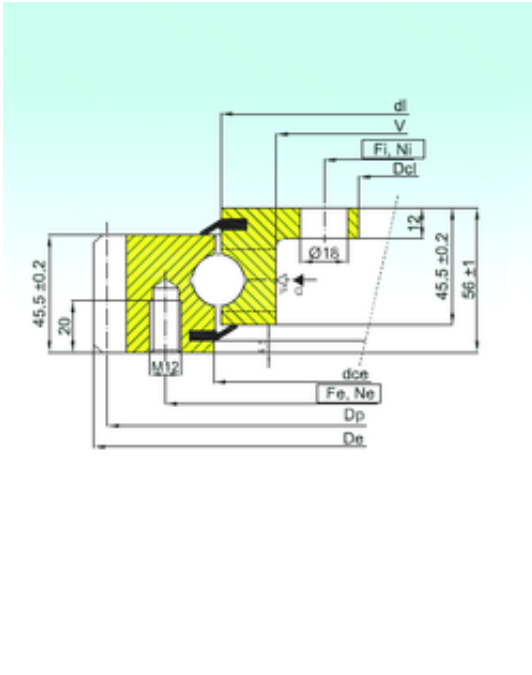
EBL.20.0744.201-2STPN Bearing 2D drawings and 3D CAD models
